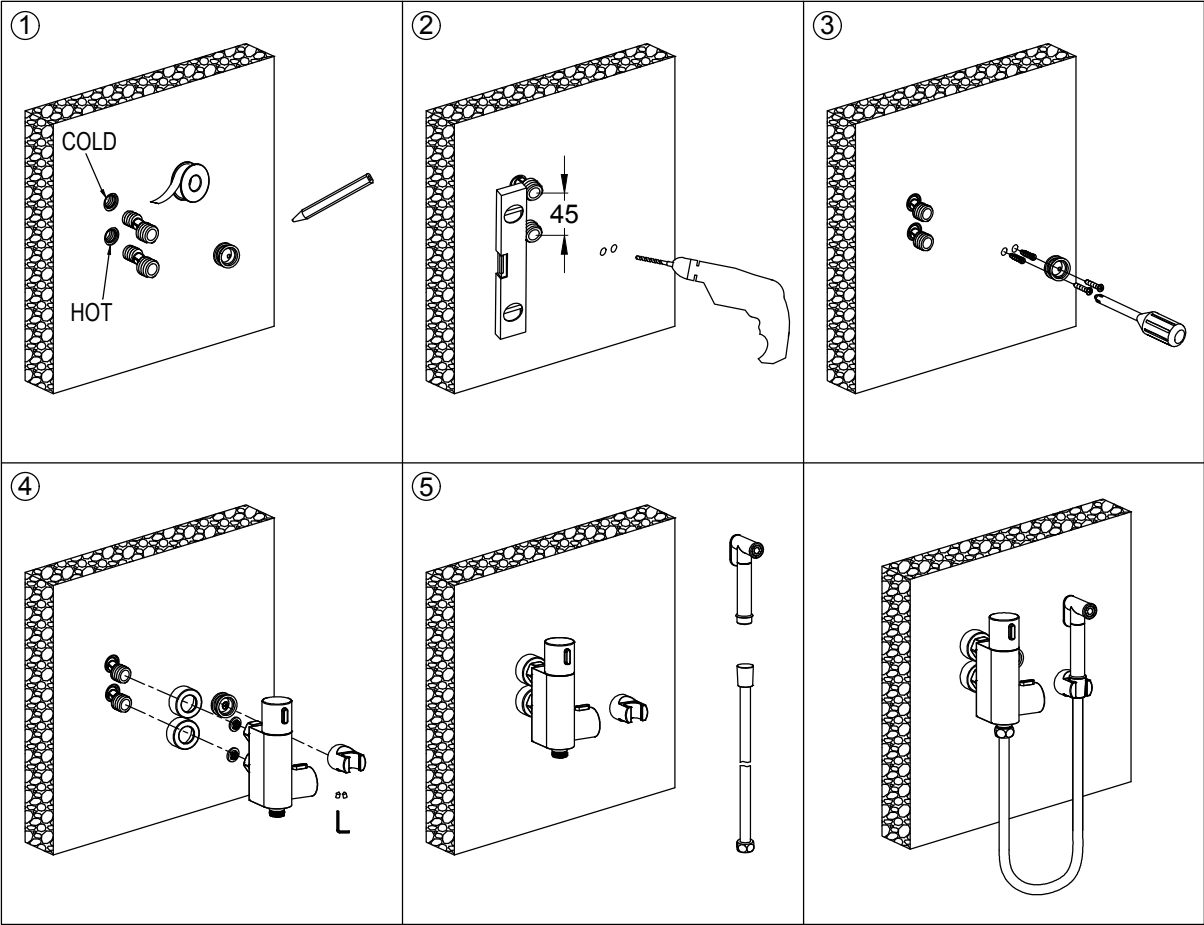
Technical drawing
