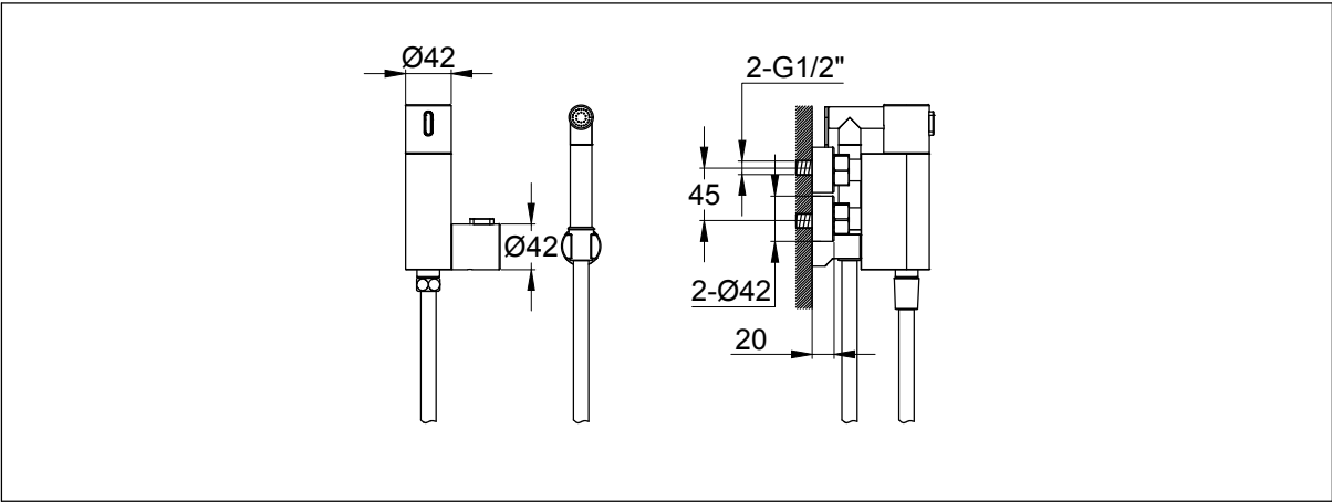
Technical drawing
