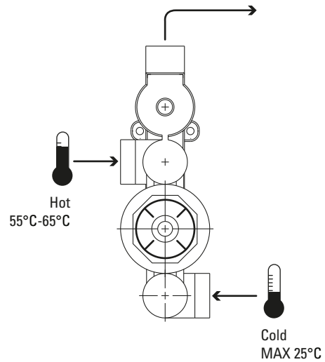
2 handles valve
