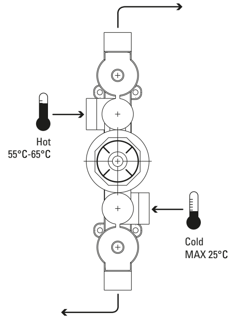
3 handles valve
