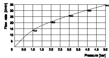
FLOW RATE CURVES
