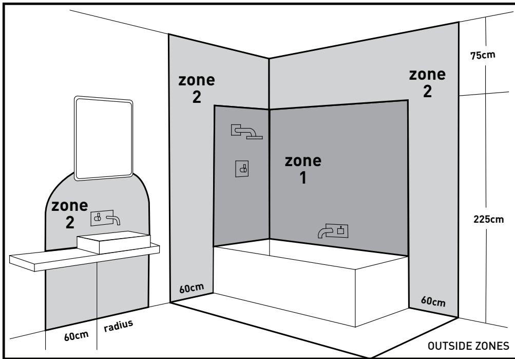
IEE Bathroom Zones Diagram
